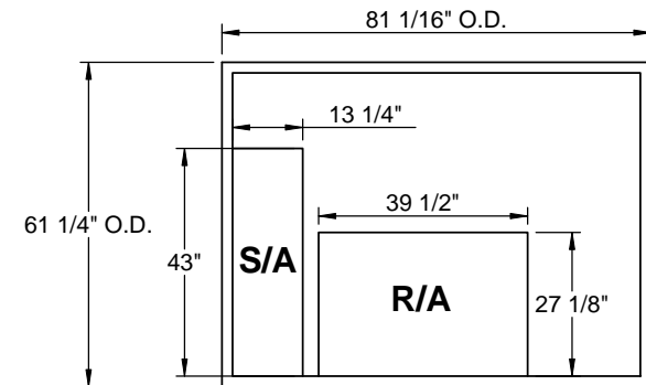
EXISTING CURB
