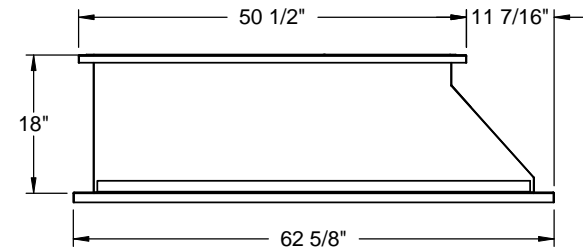
RIGHT VIEW
