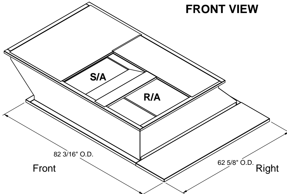
ISOMETRIC VIEW
