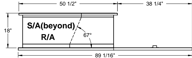
RIGHT VIEW
