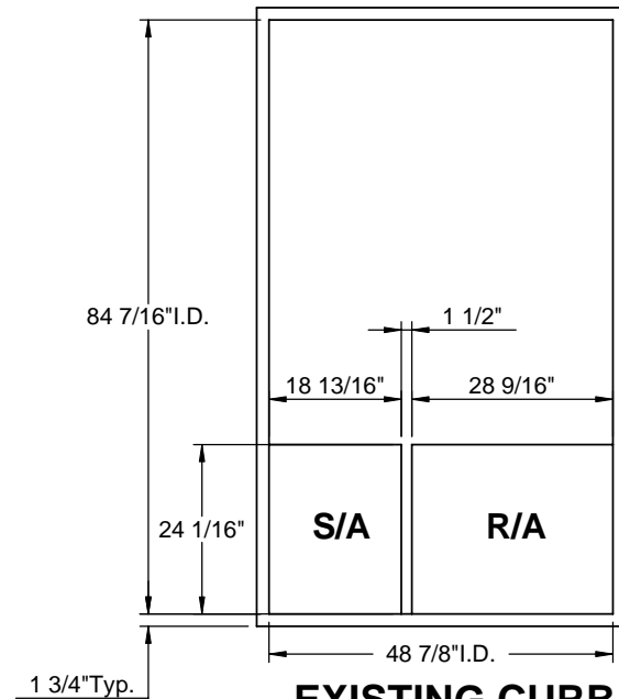
EXISTING CURB
