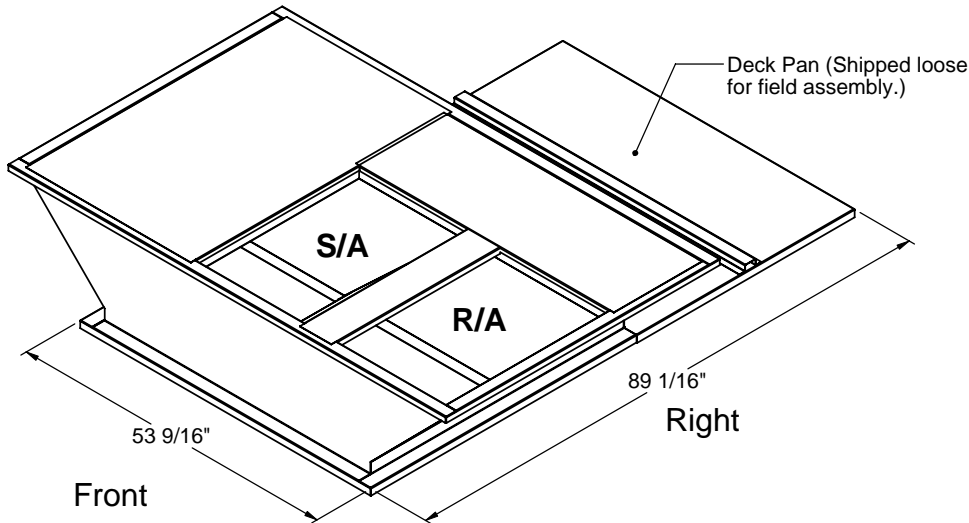
ISOMETRIC VIEW
