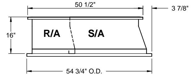
RIGHT VIEW
