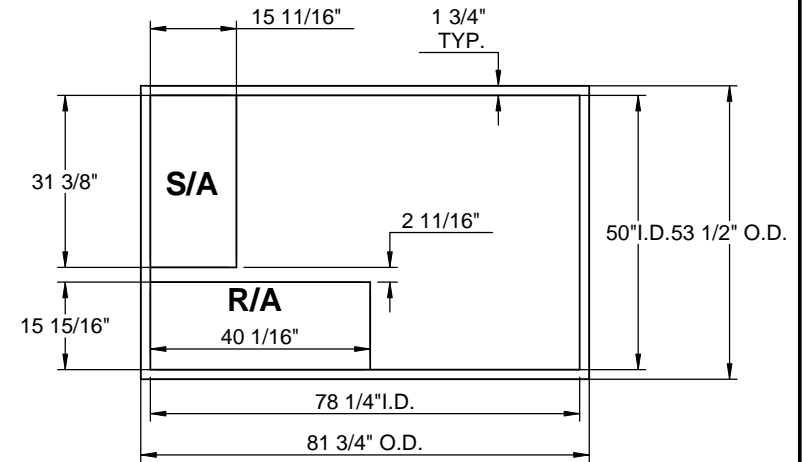
EXISTING CURB
