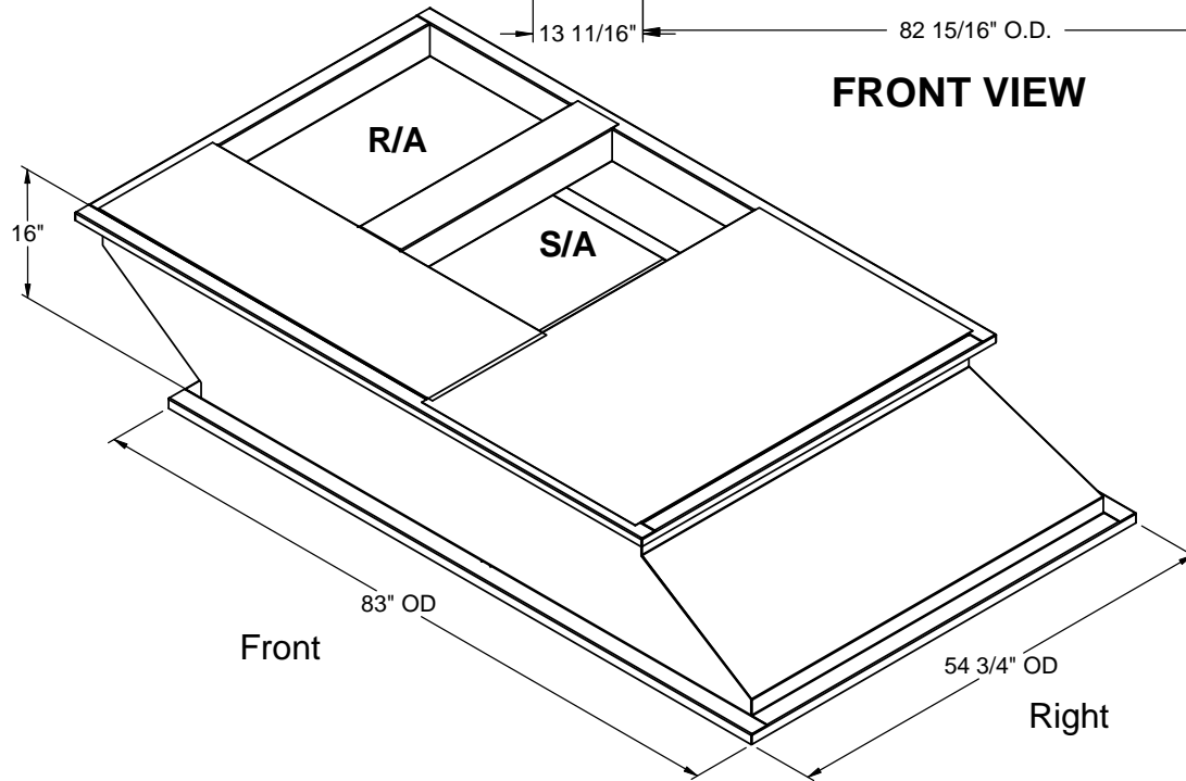
ISOMETRIC VIEW
