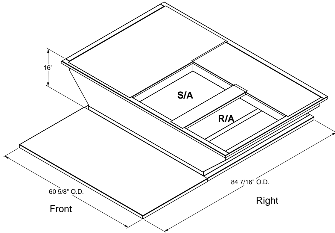
ISOMETRIC VIEW
