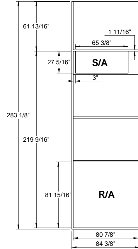
EXISTING CURB
