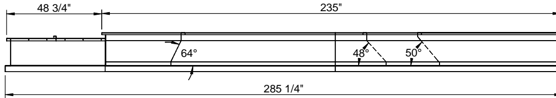
RIGHT VIEW
