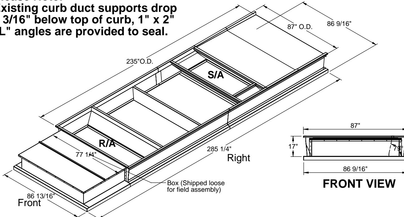
ISOMETRIC VIEW
