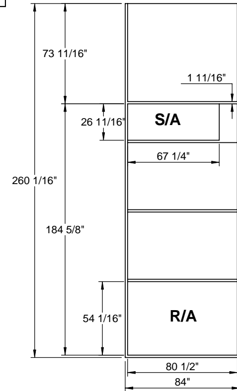
EXISTING CURB
