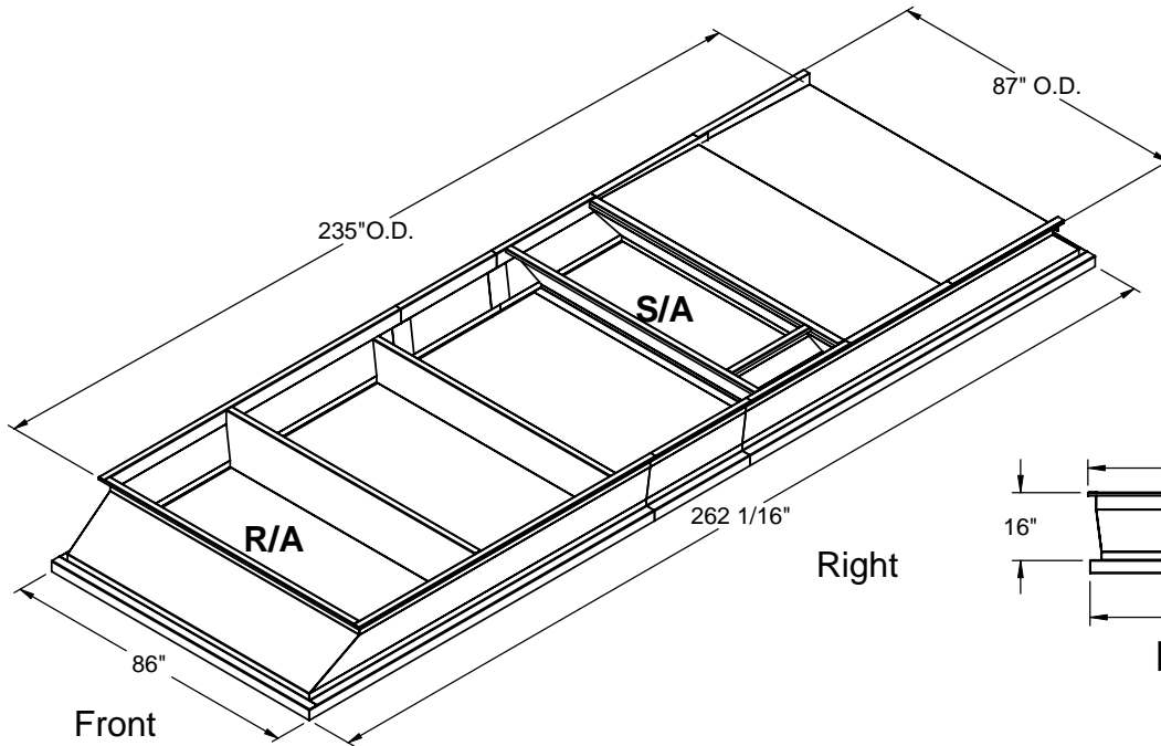
ISOMETRIC VIEW
