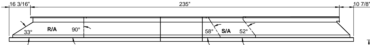
RIGHT VIEW
