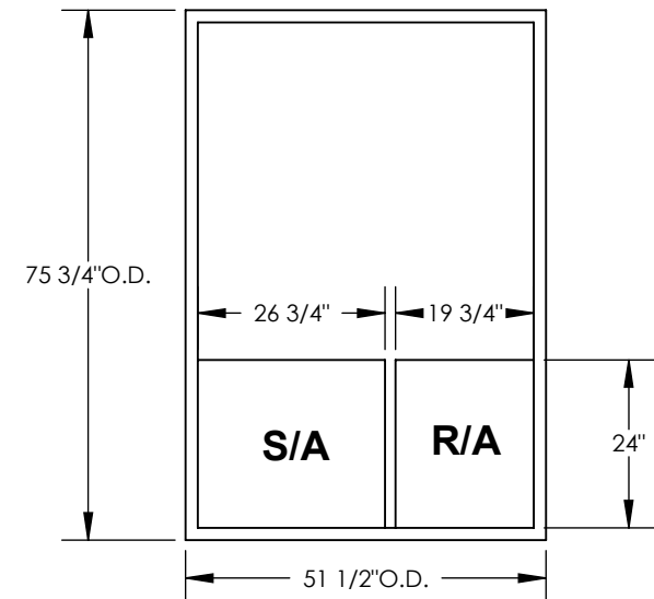
EXISTING CURB
