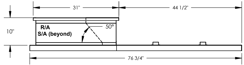
RIGHT VIEW
