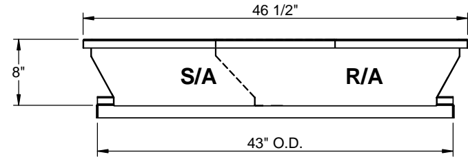
RIGHT VIEW
