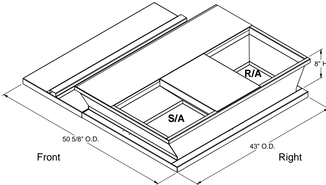
ISOMETRIC VIEW
