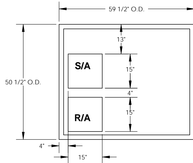
EXISTING CURB
