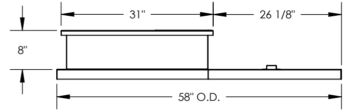
RIGHT VIEW
