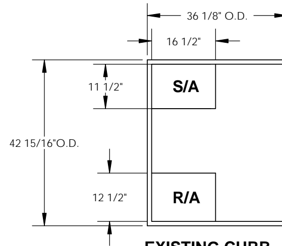
EXISTING CURB
