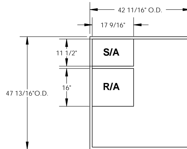
EXISTING CURB
