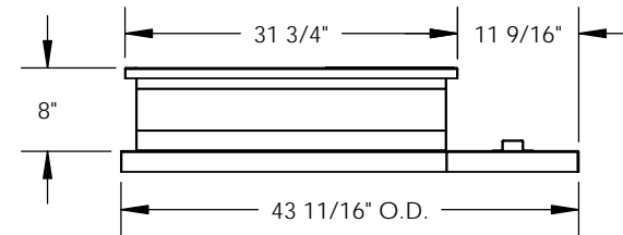
RIGHT VIEW
