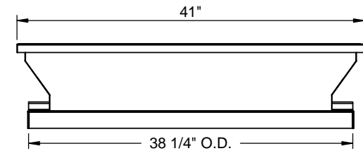
RIGHT VIEW
