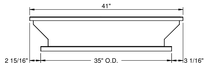
RIGHT VIEW
