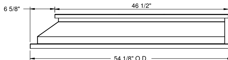
FRONT VIEW
