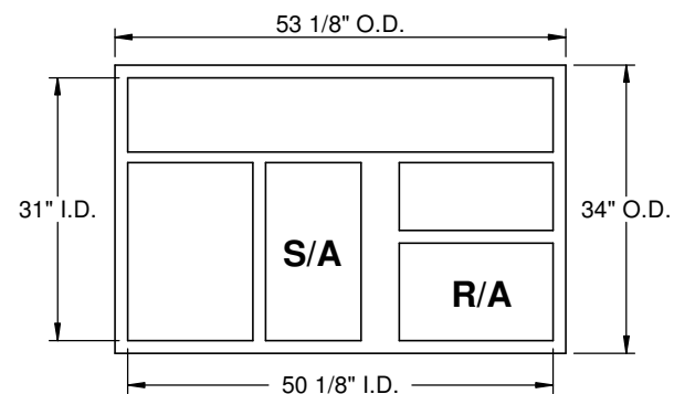
EXISTING CURB
