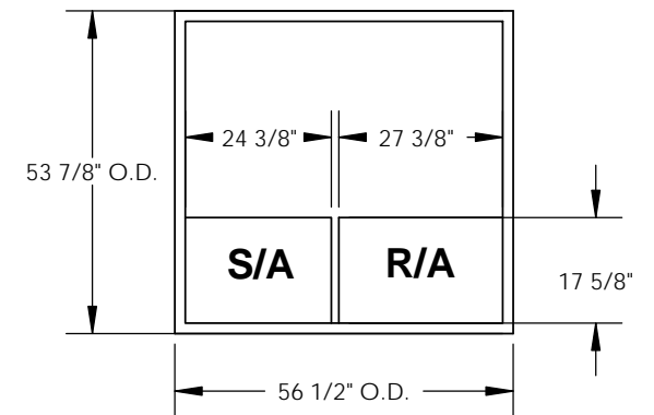
EXISTING CURB
