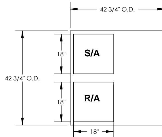
EXISTING CURB
