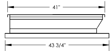
RIGHT VIEW
