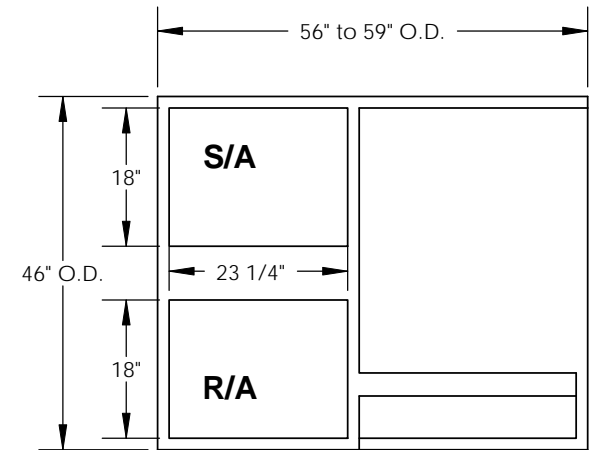
EXISTING CURB
