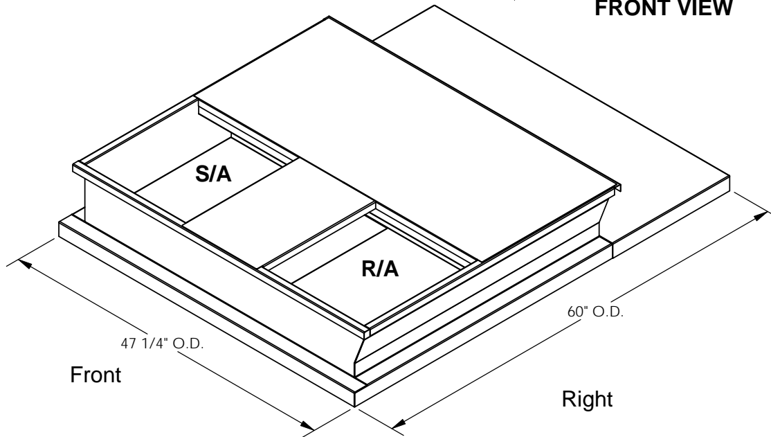
ISOMETRIC VIEW
