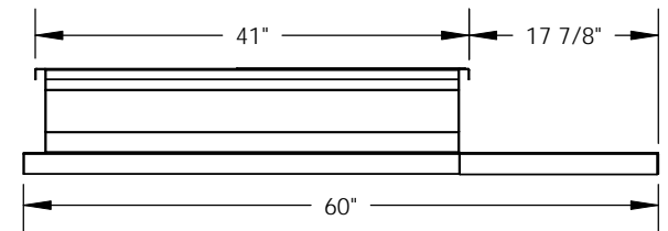
RIGHT VIEW
