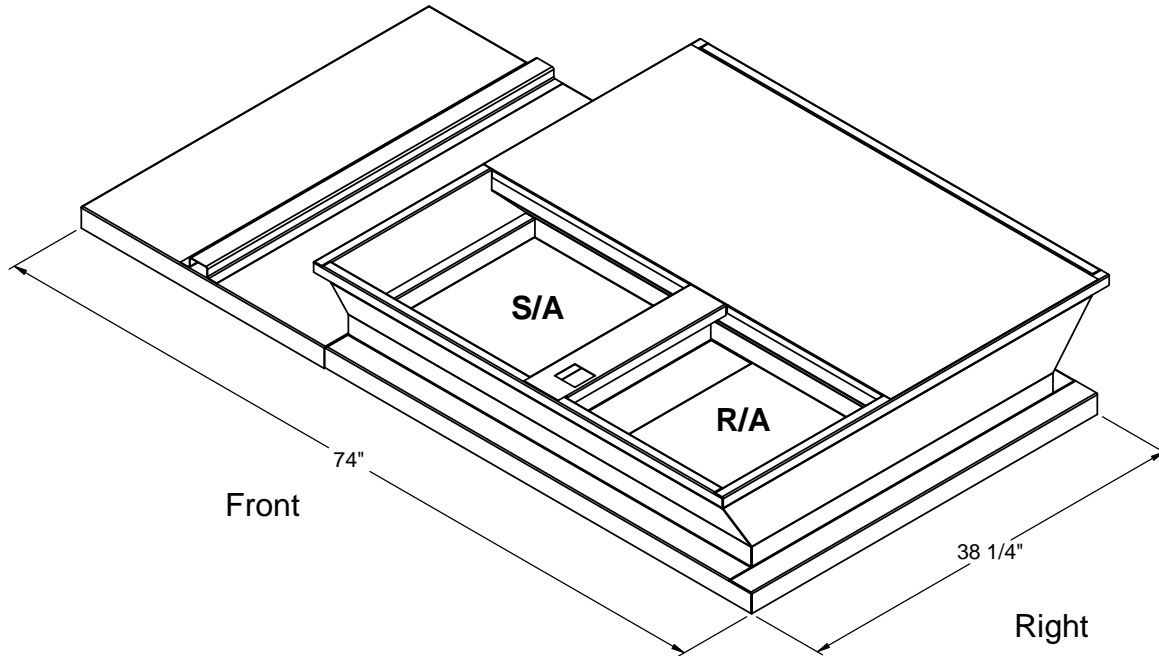
ISOMETRIC VIEW
