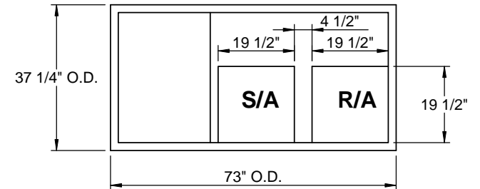
EXISTING CURB
