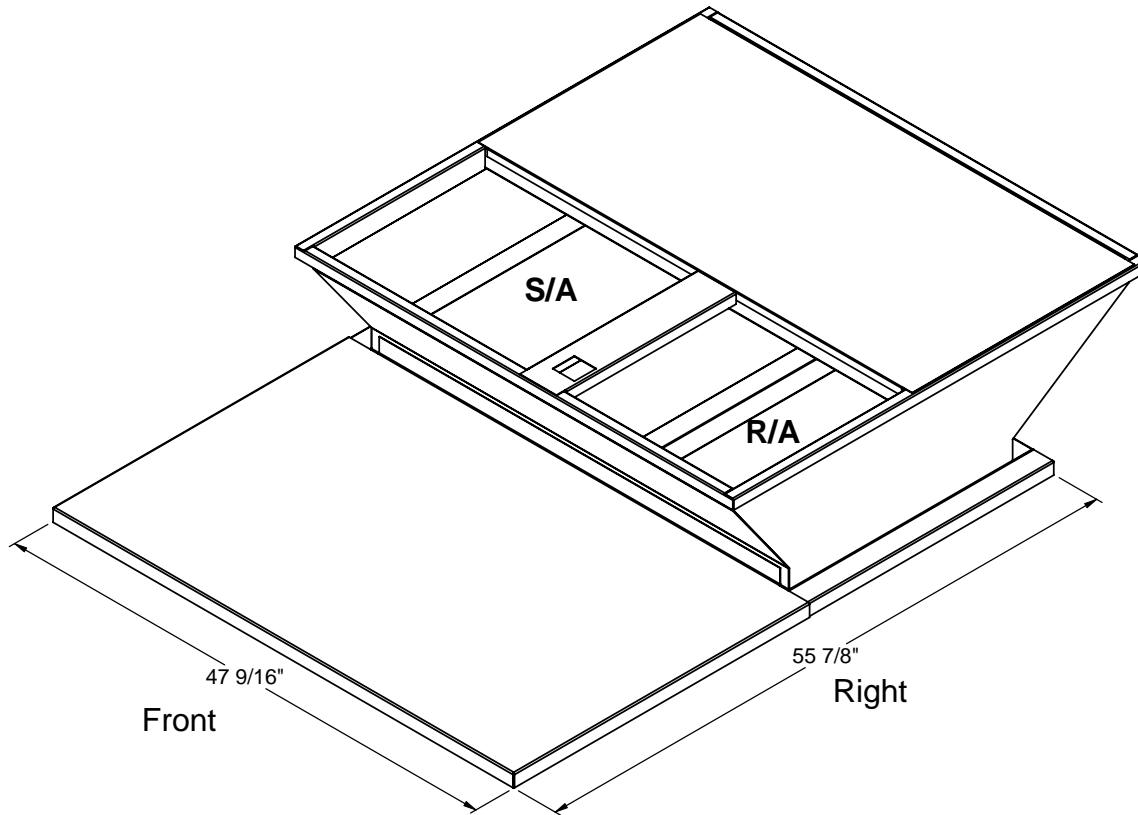
ISOMETRIC VIEW
