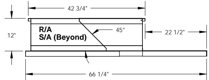
RIGHT VIEW
