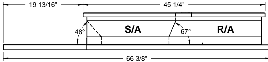
FRONT VIEW
