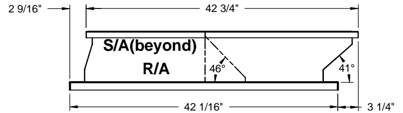
RIGHT VIEW
