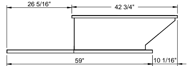
RIGHT VIEW
