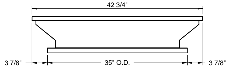
RIGHT VIEW
