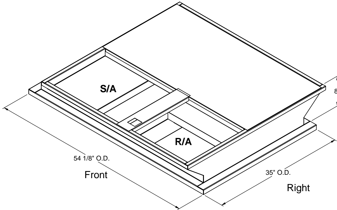
ISOMETRIC VIEW
