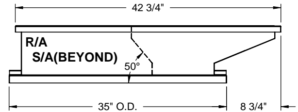
RIGHT VIEW
