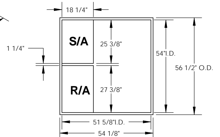
EXISTING CURB
