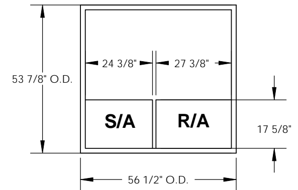
EXISTING CURB
