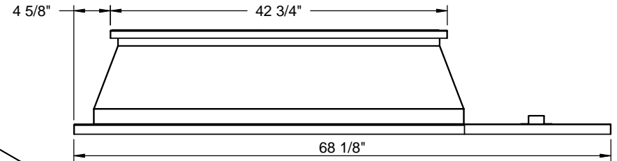
RIGHT VIEW
