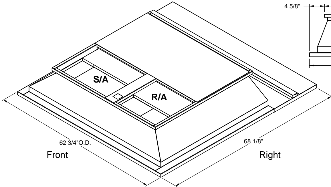
ISOMETRIC VIEW
