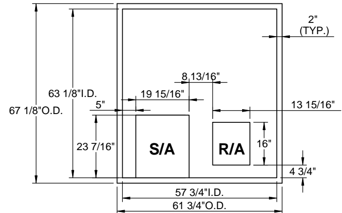
EXISTING CURB
