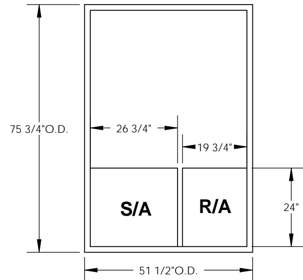
EXISTING CURB
