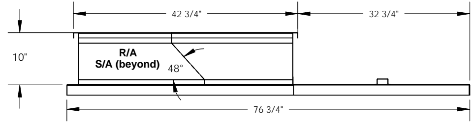
RIGHT VIEW
