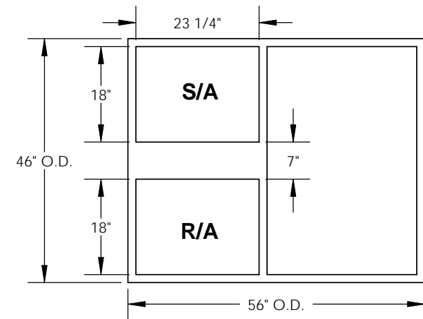
EXISTING CURB
