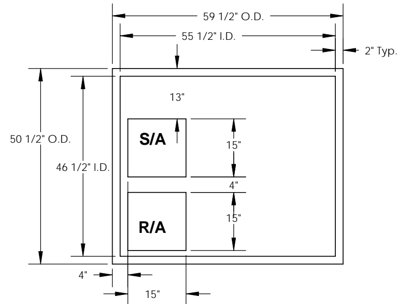
EXISTING CURB
