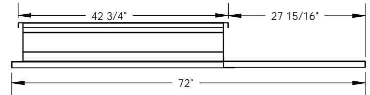
RIGHT VIEW
