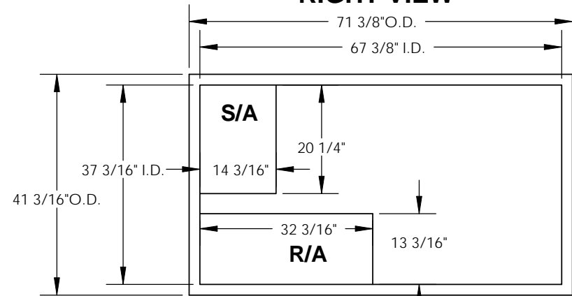
EXISTING CURB
