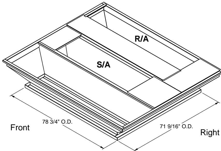
ISOMETRIC VIEW
