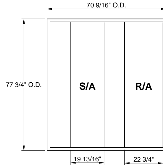
EXISTING CURB
