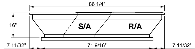
RIGHT VIEW
