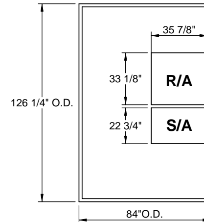
EXISTING CURB
