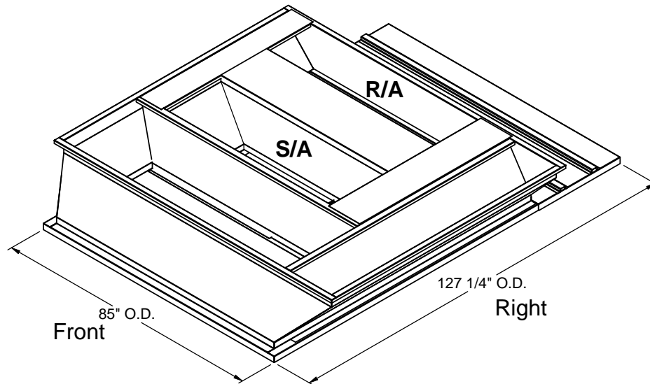
ISOMETRIC VIEW
