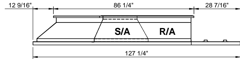
RIGHT VIEW
