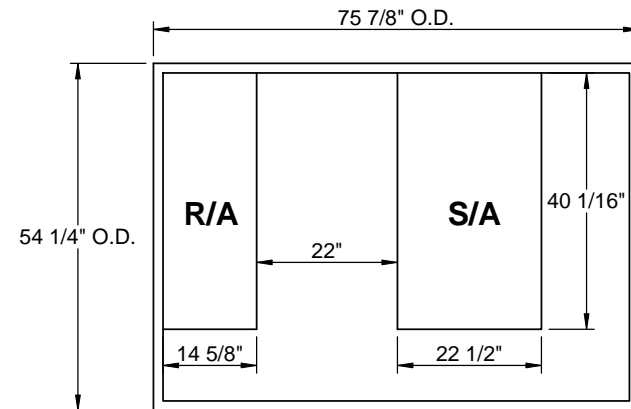
EXISTING CURB
