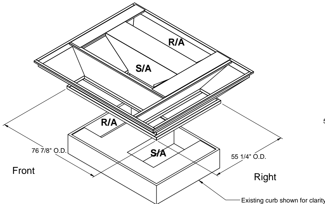
ISOMETRIC VIEW
