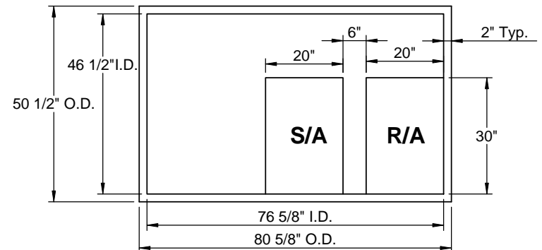
EXISTING CURB
