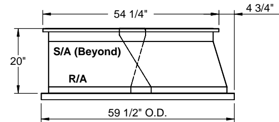
RIGHT VIEW
