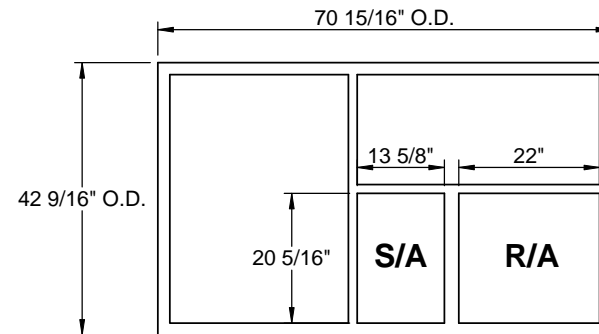
EXISTING CURB
