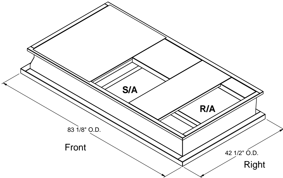
ISOMETRIC VIEW
