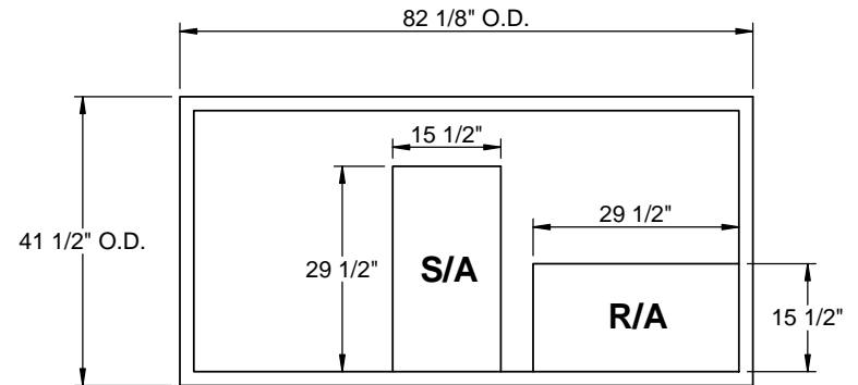
EXISTING CURB
