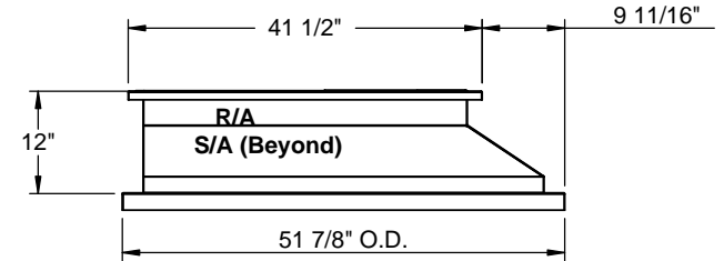
RIGHT VIEW
