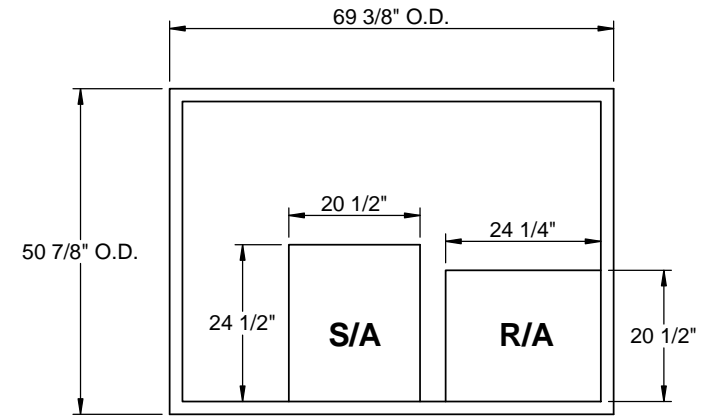
EXISTING CURB
