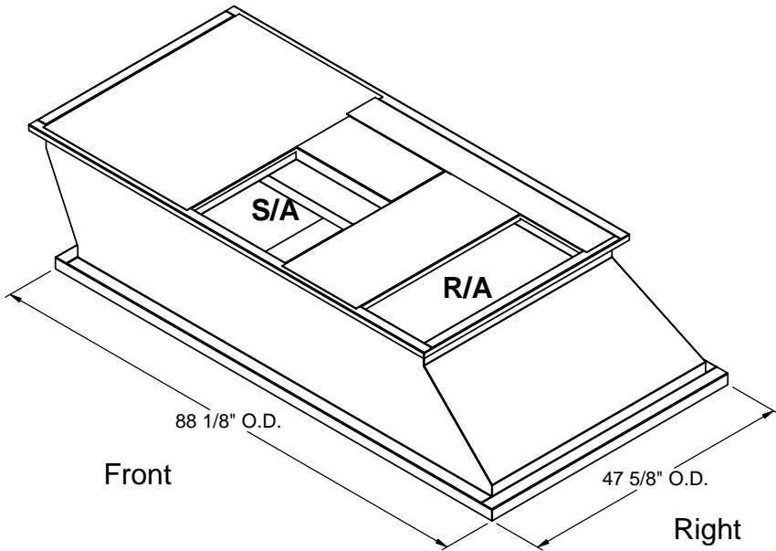
ISOMETRIC VIEW
