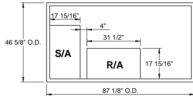
EXISTING CURB
