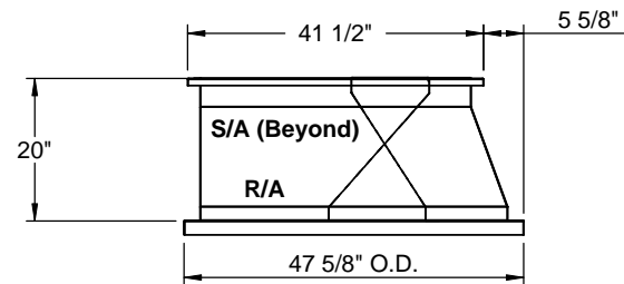
RIGHT VIEW
