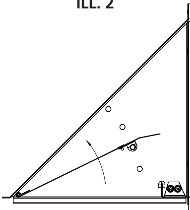
Manual Fixed Blade Position Setpoint OAMANSUN3672 Series
